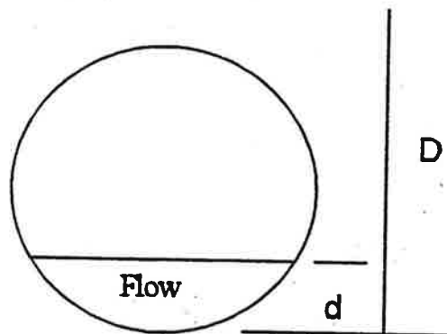
Figure 16: "D" is the diameter of the pipe and "d" is the depth of the flow. The wetted perimeter is that portion of the circumference submerged with water and the dry perimeter is the portion of the circumference above the water line.
