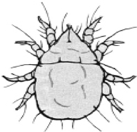
Figure 2.18 Grain mite
