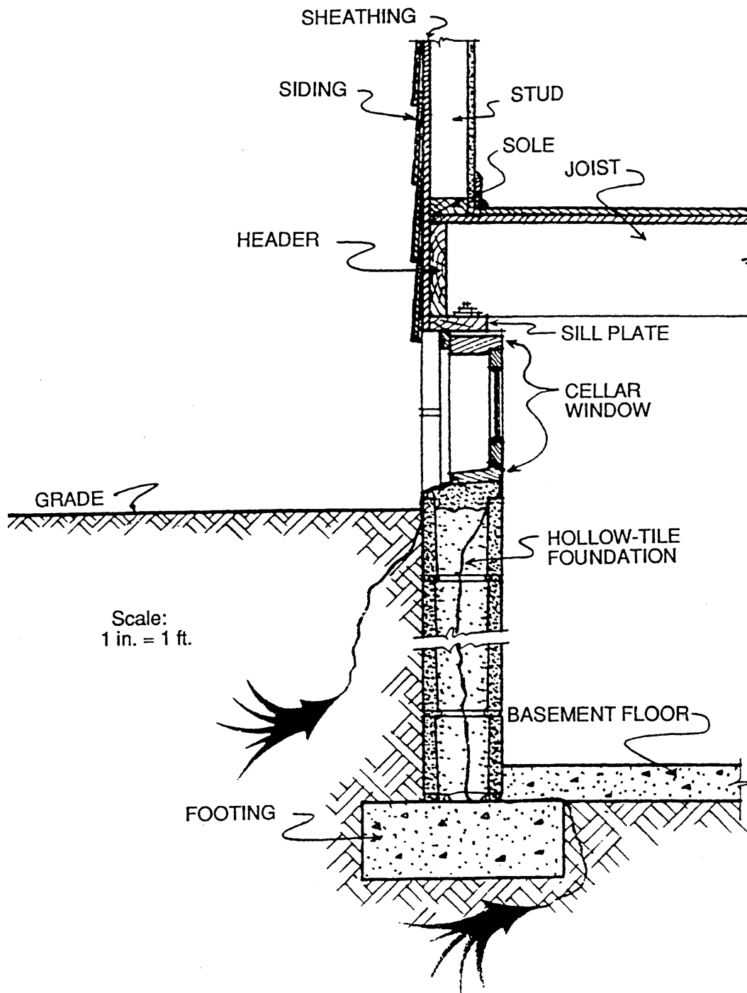
Concrete Block Foundation
